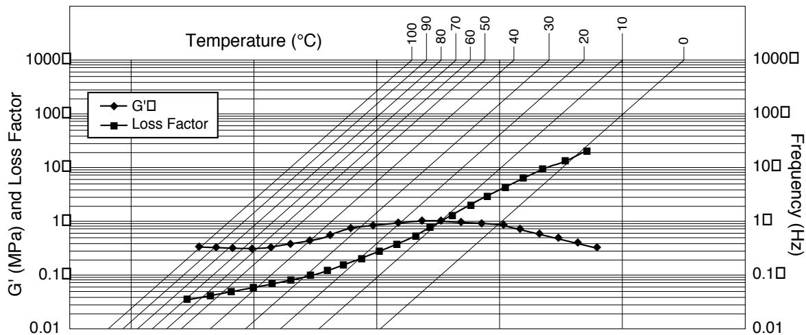
3M™ Ultra-Pure Viscoelastic Damping Polymer 242 Nomograph
