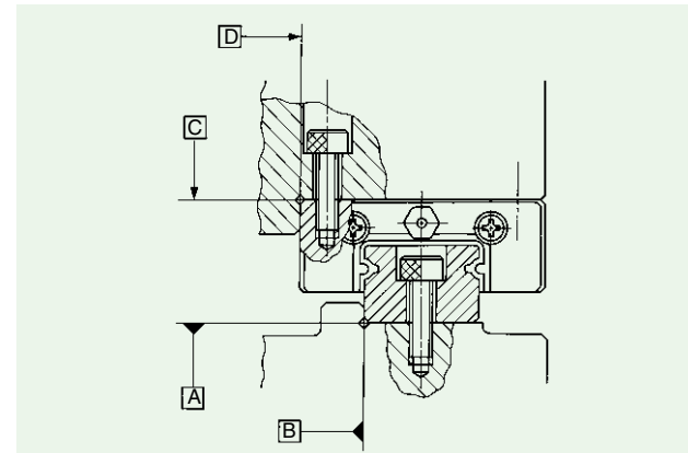
Fig. 4 Reference mounting surfaces and general mounting structure
