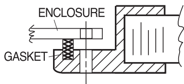
Figure 5 - Style 3036 Recess Mount
