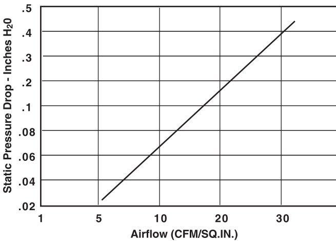
Figure 3 - Style 3031 Through Hole
